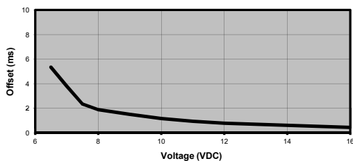
Voltage Sensitivity Summary, 6-16V
