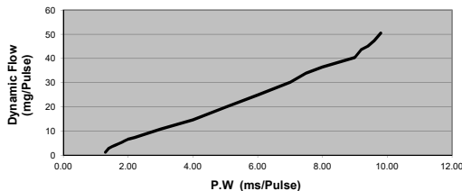
Characteristic Injector Flow Curve
